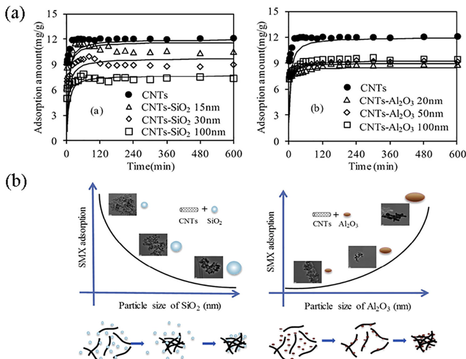
Fig. 8. (a) Adsorption kinetics of SMX on CNT in the absence and presence of \text{SiO}_2 (left) and \text{Al}_2\text{O}_3 (right). (b) Effect of size and the type nanoparticles for removal of SMX by CNT. Reproduced with permission from Ref. [125]. Copyright 2017, Elsevier.
