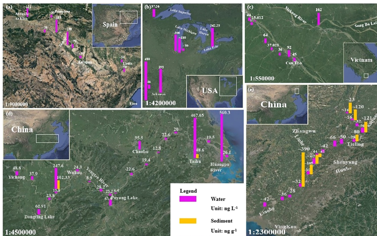
Fig. 1. The distribution of total SNs in rivers and sediments. (a) Ebro River basin, (b) Lake Erie, Southern Lake Michigan, Skaneateles Lake and Arkansas surface water, (c) Mekong River, (d) Yangtze River basin, (e) Liaohe River. The column chart represents the general distribution of the total concentration of SNs in water and sediments, respectively. The height of the column chart represents the level of total SNs concentration. The numerical data are from [11,40,42–47].
