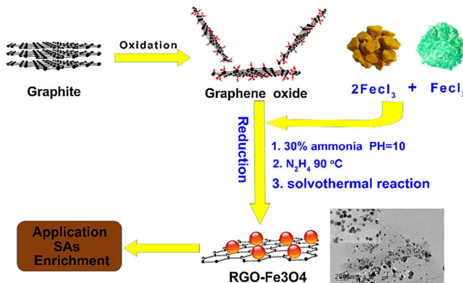
Fig. 3. Synthetic schematic for Fe 3 O 4 -GO. Reproduced with permission from Ref. [100]. Copyright 2016, Elsevier.
