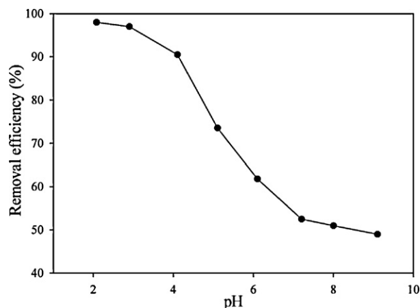
Fig. 6. Effect of pH on removal of Cr(VI) (metal concentration 100 \text{ mg L}^{-1} , adsorbent dose 0.08 \text{ g} , contact time 30 \text{ min} , temperature 25^\circ\text{C} ).
